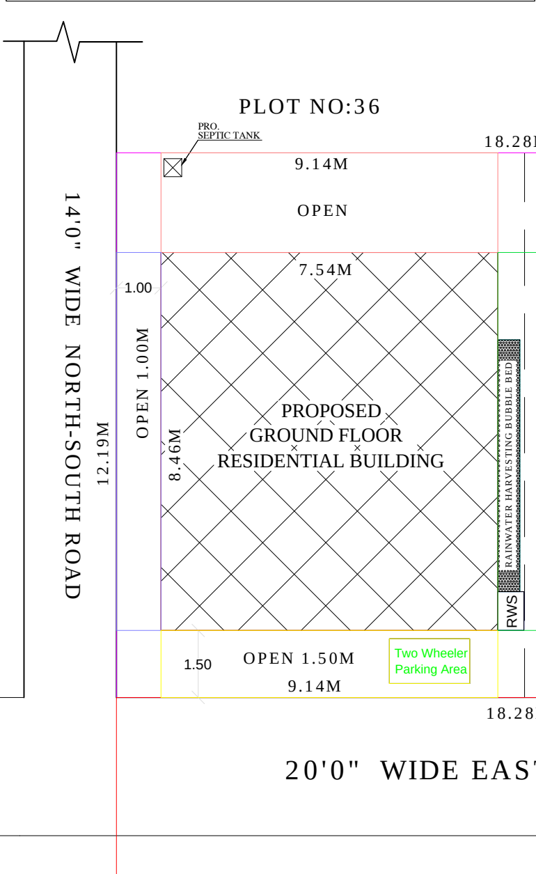
SITE PLAN (SCALE 1:1)
