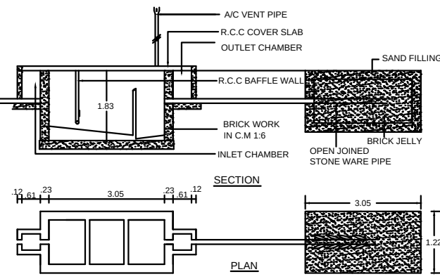
DETAILS OF SEPTIC TANK AND DISPERSION TRENCH
