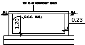
RWH_CAPACITY_L=2000LTRS
