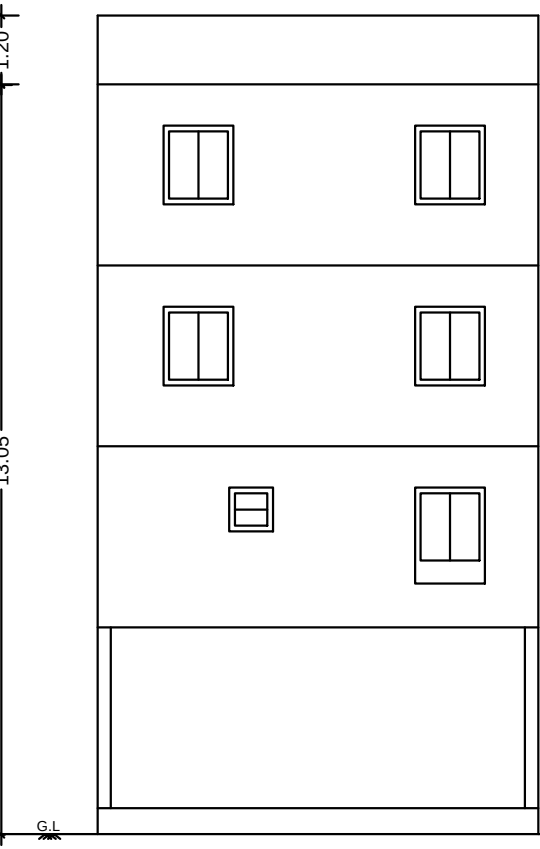
FRONT ELEVATION
