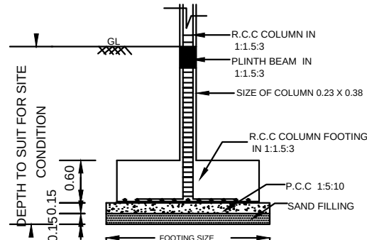
FOUNDATION DETAILS NOT TO SCALE
