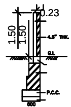
COMPOUND DETAIL
