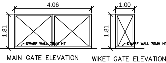
MAIN GATE ELEVATION WICKET GATE ELEVATION
