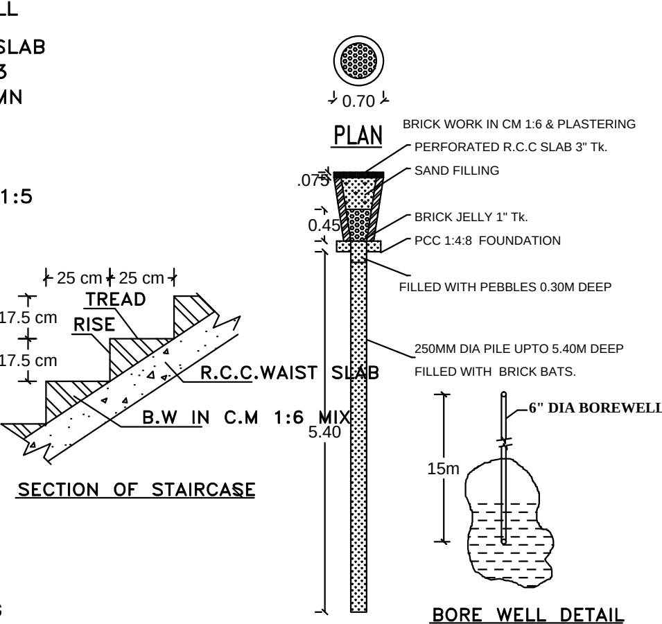
SECTION OF RAIN WATER PERCOLATION PIT
