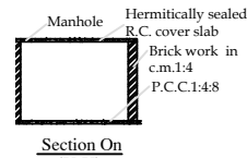
Section On 'Y-Y'
