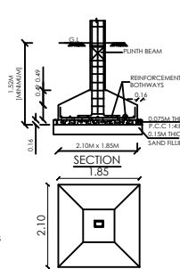
FOUNDATION DETAILS
