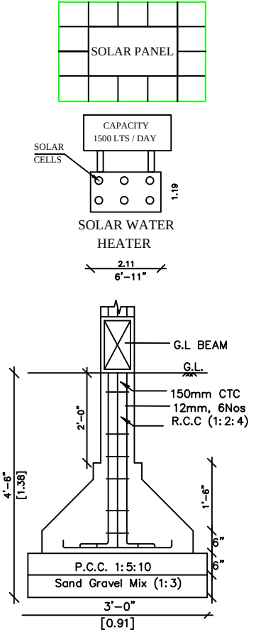
R.C.C. COLUMN FOOTING DETAILS
