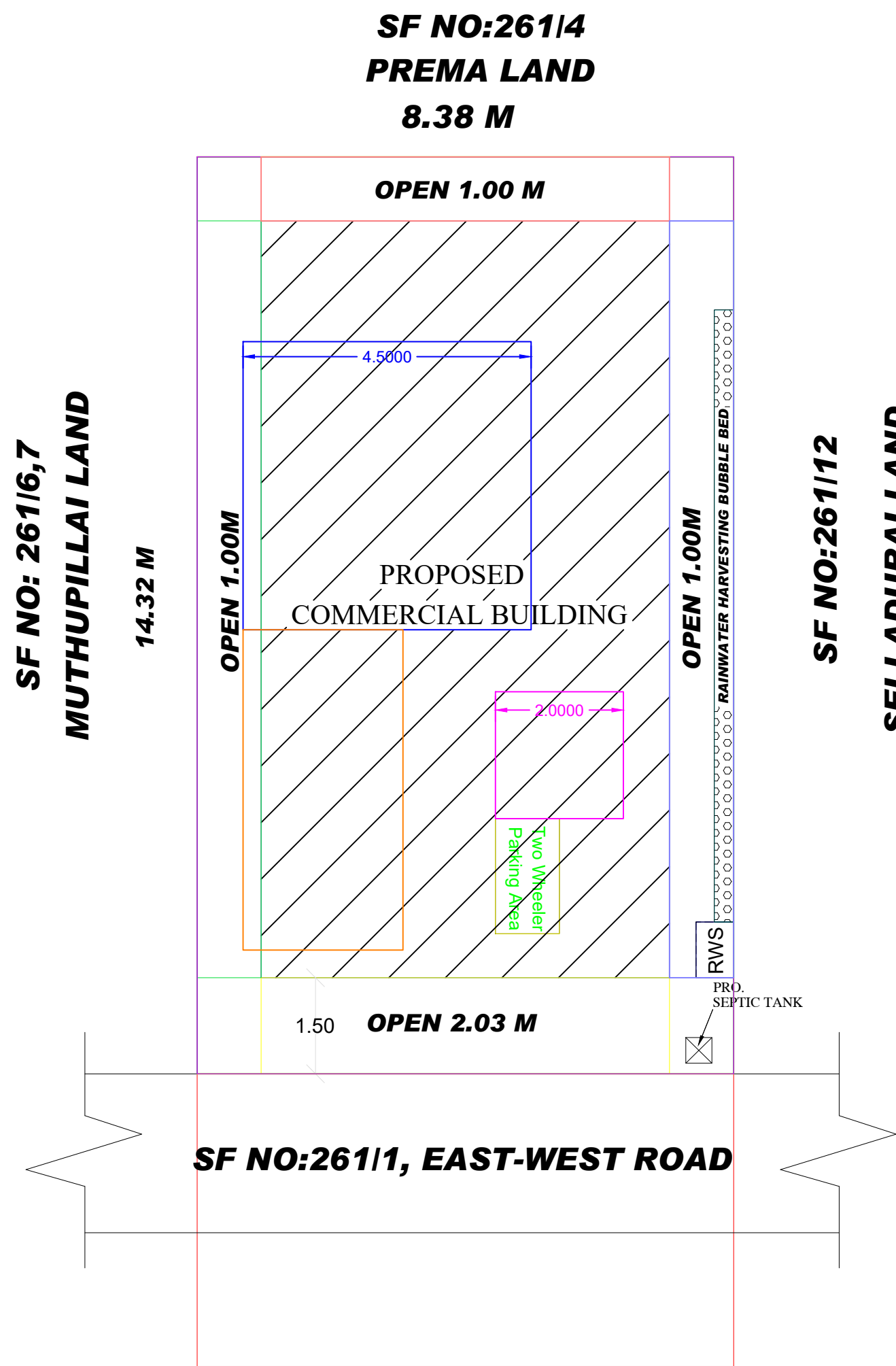
SITE PLAN (SCALE 1:1)
