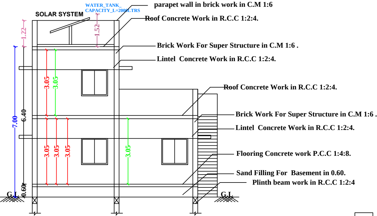
SECTION-AB
