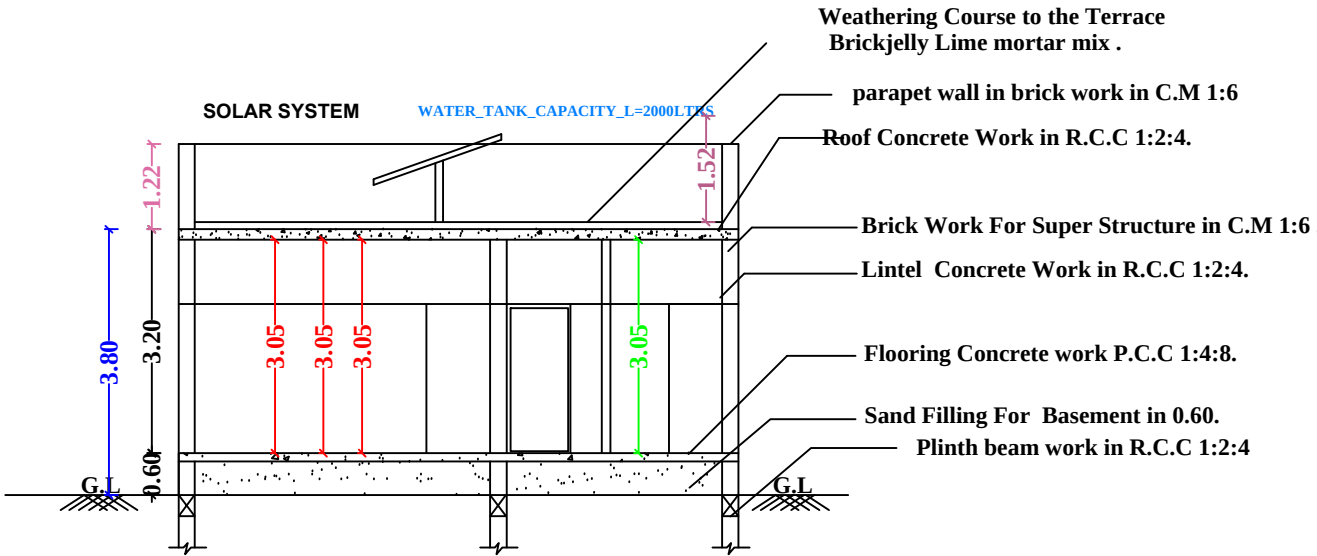
SECTION-AB
