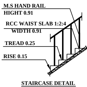
STAIRCASE DETAIL
