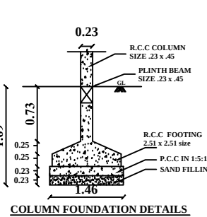
COLUMN FOUNDATION DETAILS
