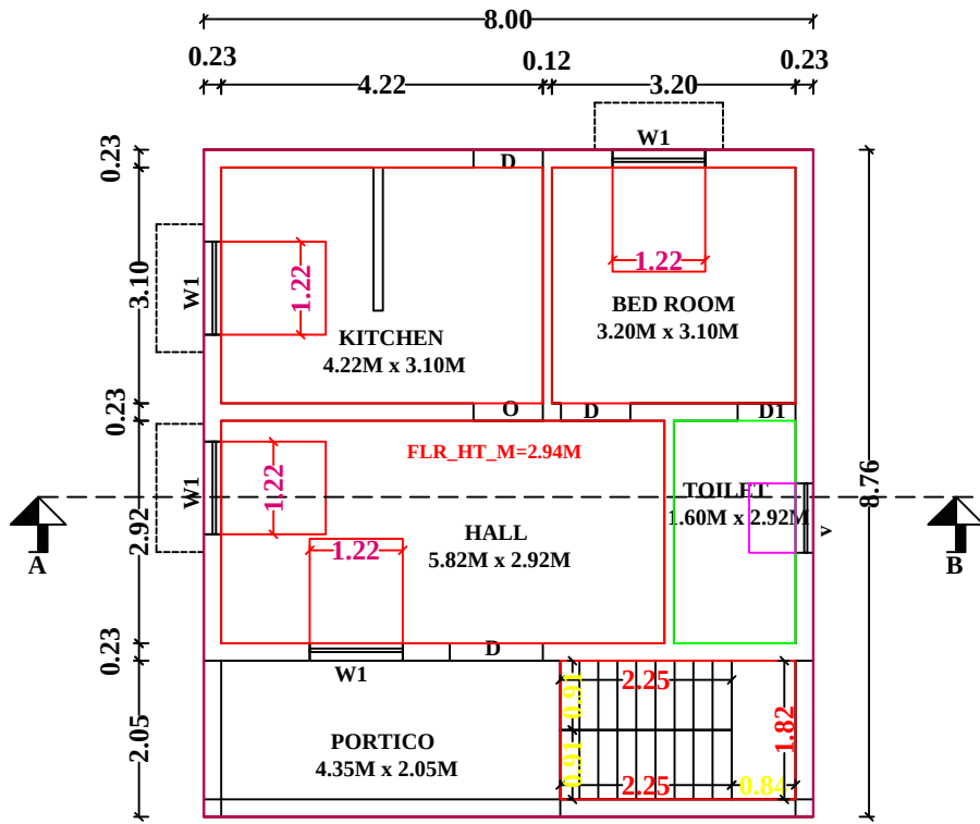
FLOOR-0 PRO.GROUND FLOOR PLAN
