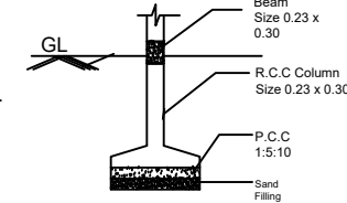
FOUNDATION DETAILS
