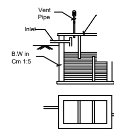
SEPTIC TANK & D-TRENCH DETAILS
