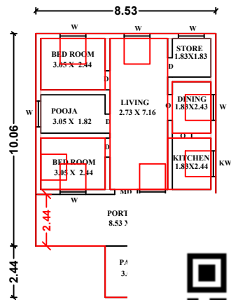
PRO.GROUND FL
