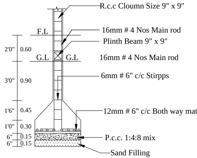
COLUMN DETAILS
