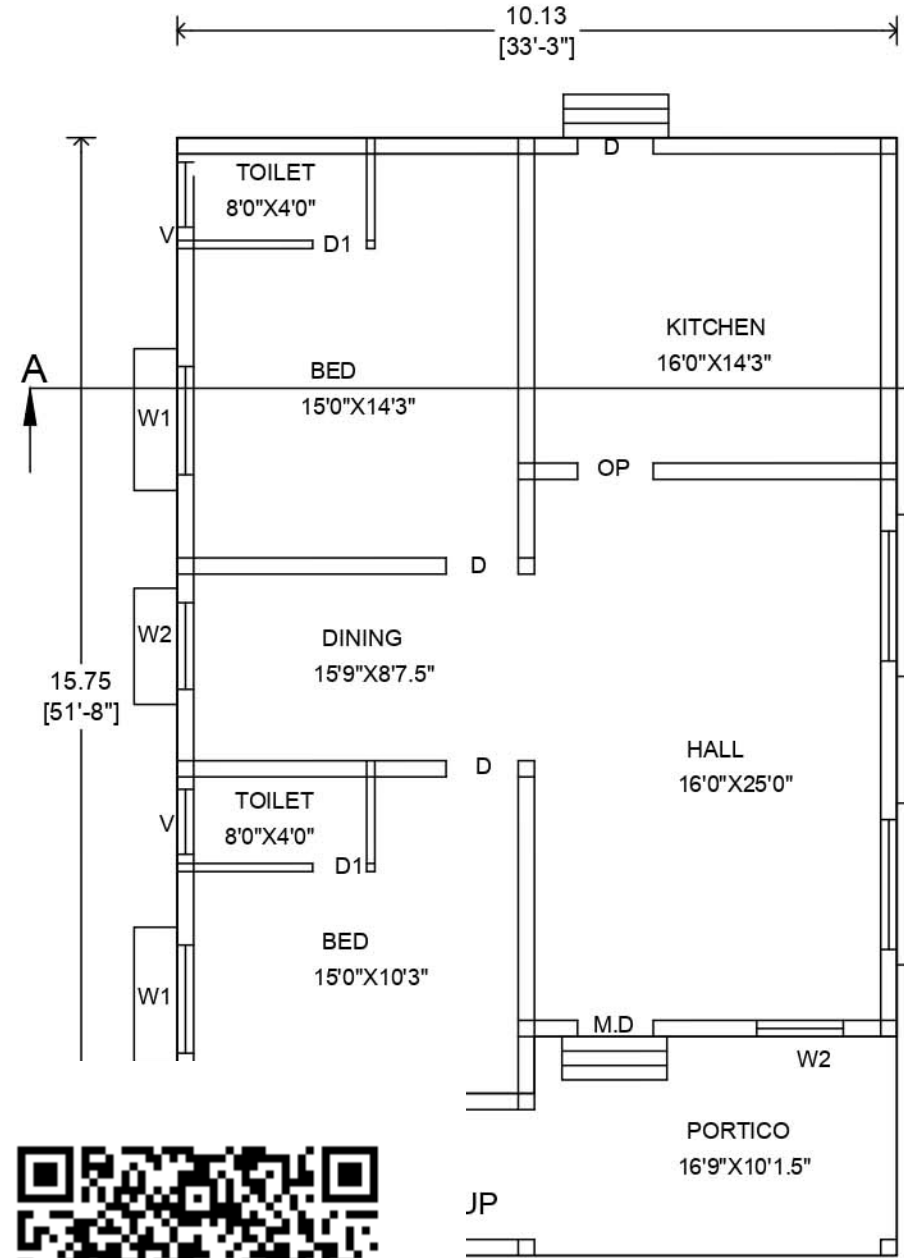
GROUND FLOOR
