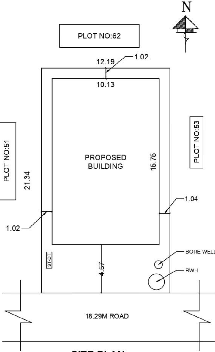
SITE PLAN
