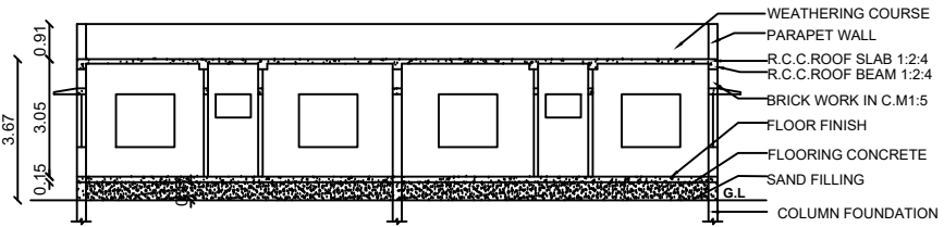
SECTION ON SS
