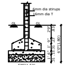
COLUMN FOUNDATION DETAIL
