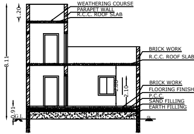
SECTION ON XX
