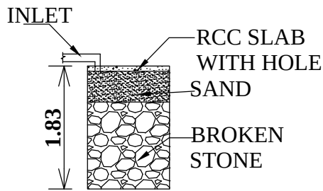
SECTION-DD
