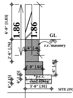
COMPOUND WALL
