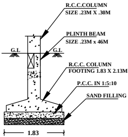
COLUMN DETAILS
