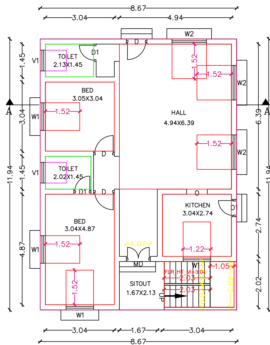
OR PLAN
