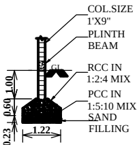
COLUMN DETAILS
