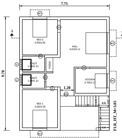
PRO GROUND FLOOR
