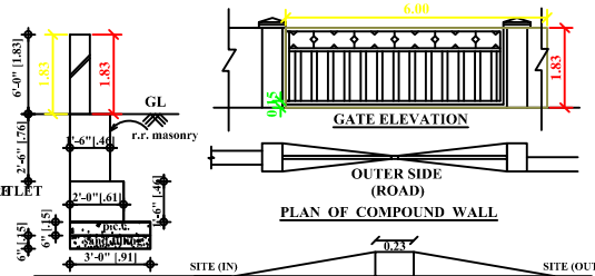
COMPOUND WALL & GATE DETAIL
