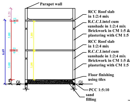
SECTION X - X
