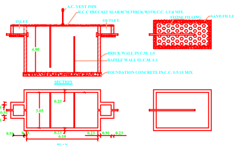
PLAN & SECTION OF SEPTIC TANK & DISPERSION TRENCH
