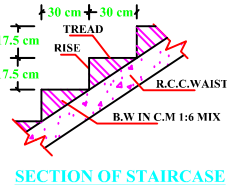
SECTION OF STAIRCASE
