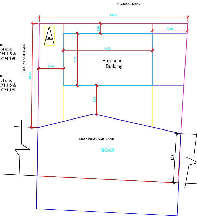
SITE PLAN
