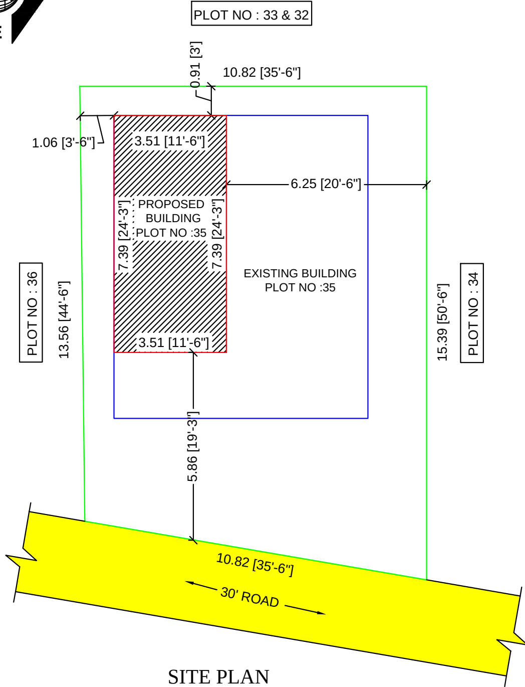
SITE PLAN
