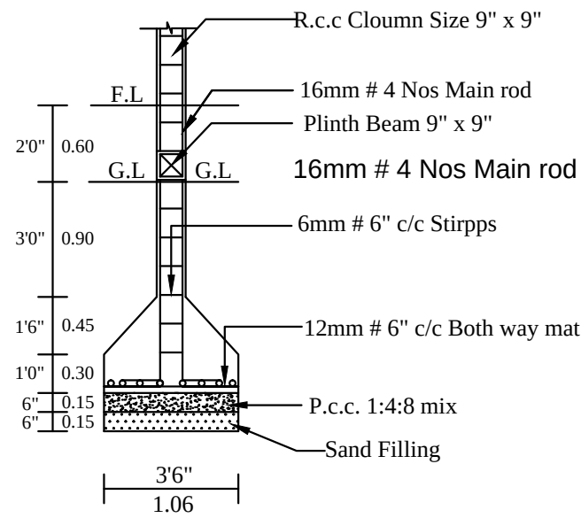
COLUMN DETIAL
