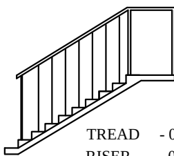
STAIRCASE DETAILS
