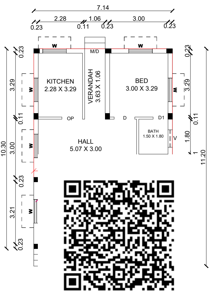
EXISTING & PROPOSED GROUND FLOOR PLAN
