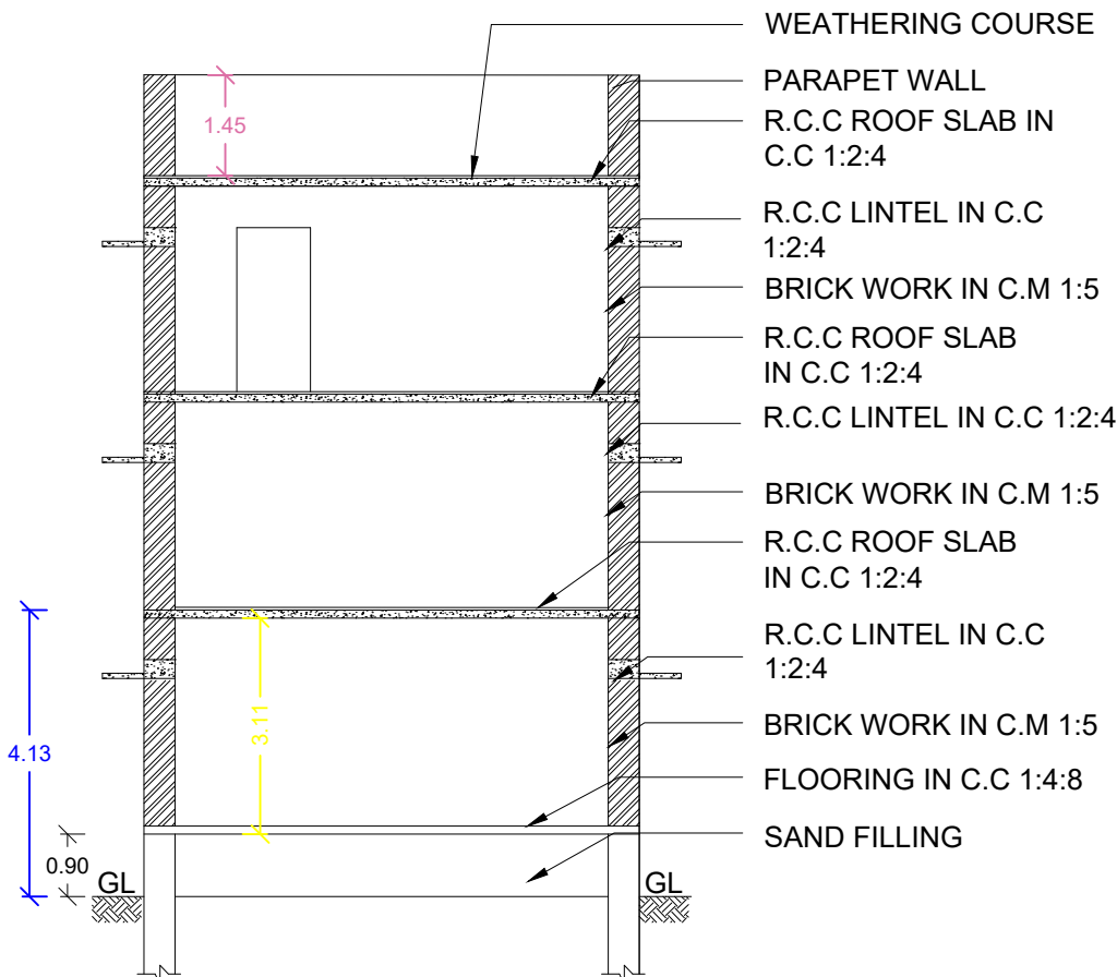
PROPOSED GROUND FLOOR BUILDING SECTION ON- AA
