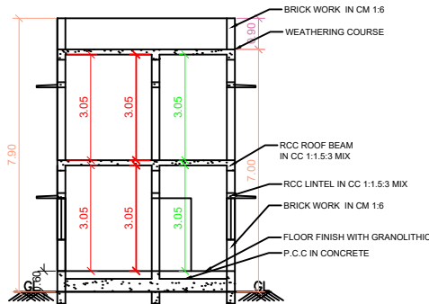
SECTION AB
