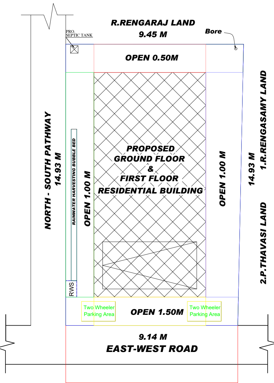
SITE PLAN (SCALE 1:1)
