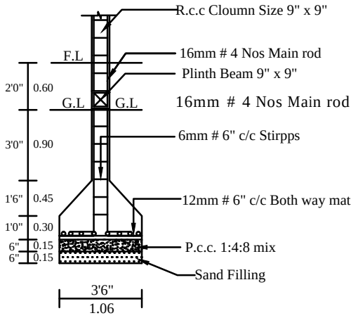
COLUMN DETIAL
