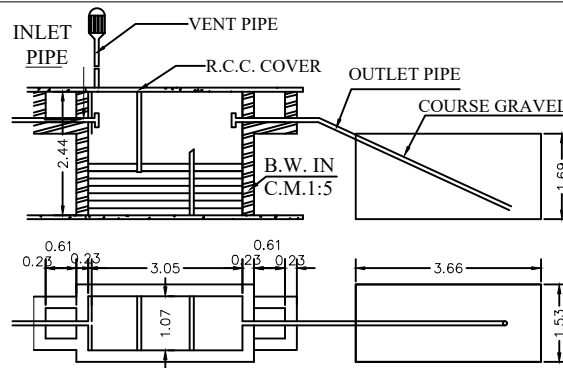
SEPTIC TANK & OF DISPERSION TRENCH DETAILS (NOT TO SCALE)
