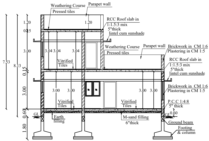
SECTION X-X
