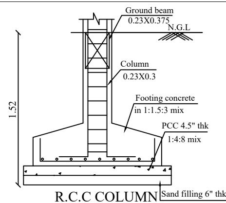
R.C.C COLUMN FOUNDATION
