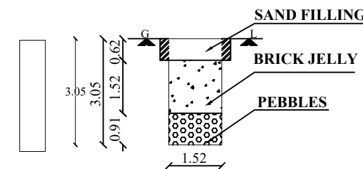
RAIN WATER HARVESTING SYSTEM RWH_CAPACITY_L=5000LTS
