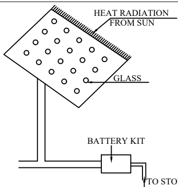
SOLAR SYSTEM (NOT TO SCALE)
