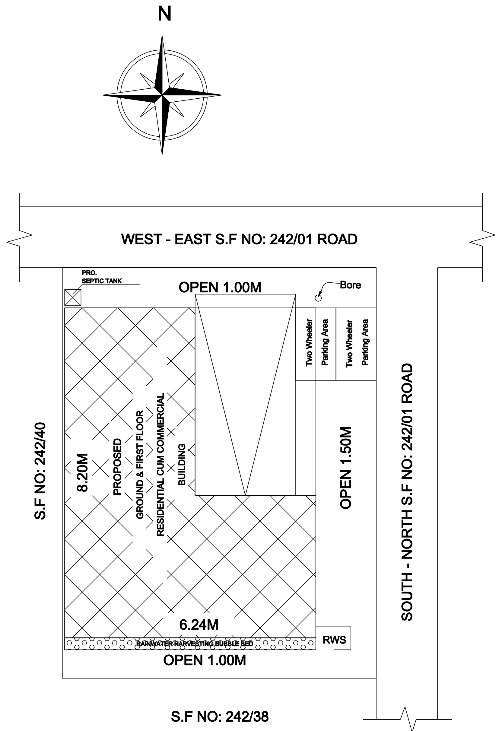
SITE PLAN
