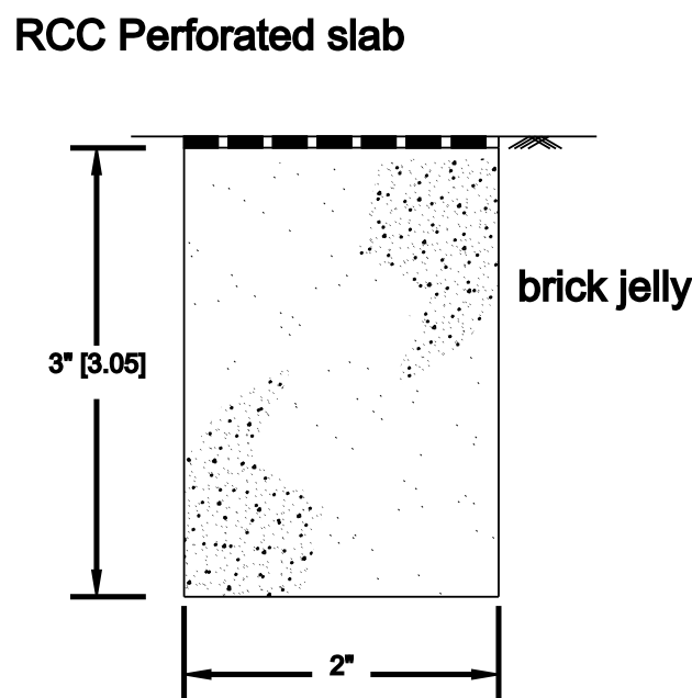
RAIN WATER PERCOLATION PIT (SCALE = 1 : 50 )
