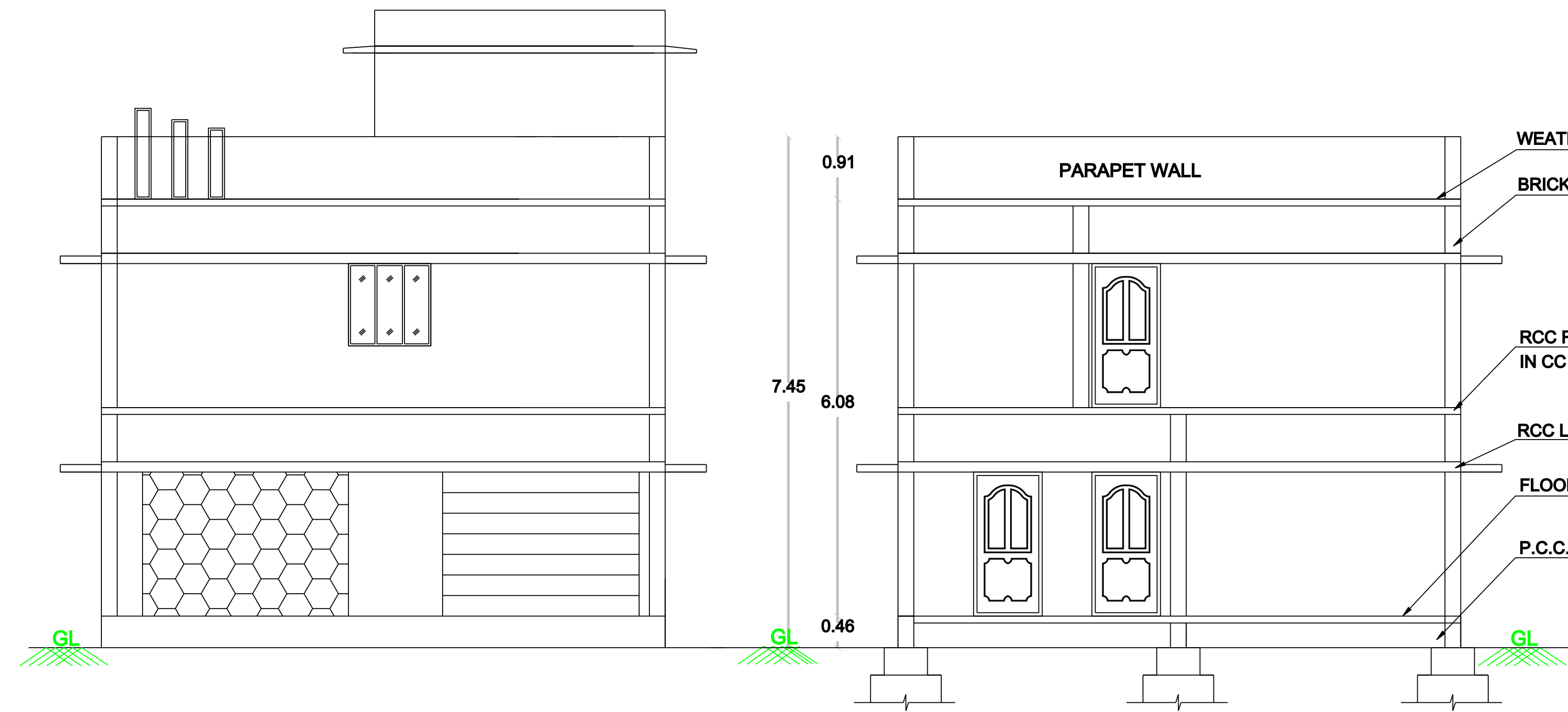
FRONT ELEVATION
