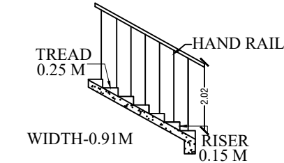
STAIRCASE DETAILS
