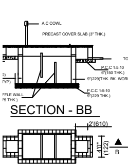
PLAN OF SEPTIC TANK
