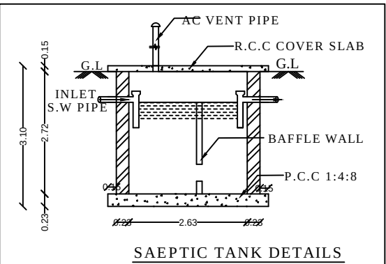
SAEPTIC TANK DETAILS
