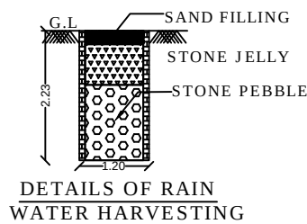
DETAILS OF RAIN WATER HARVESTING
