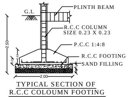
TYPICAL SECTION OF R.C.C COLOUMN FOOTING
