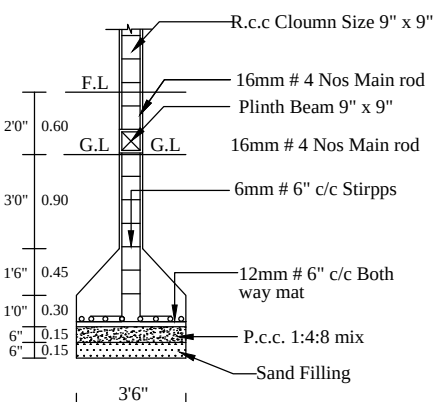
COLUMN DETAILS
