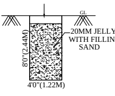
RAIN WATER HARVESTING UNIT
