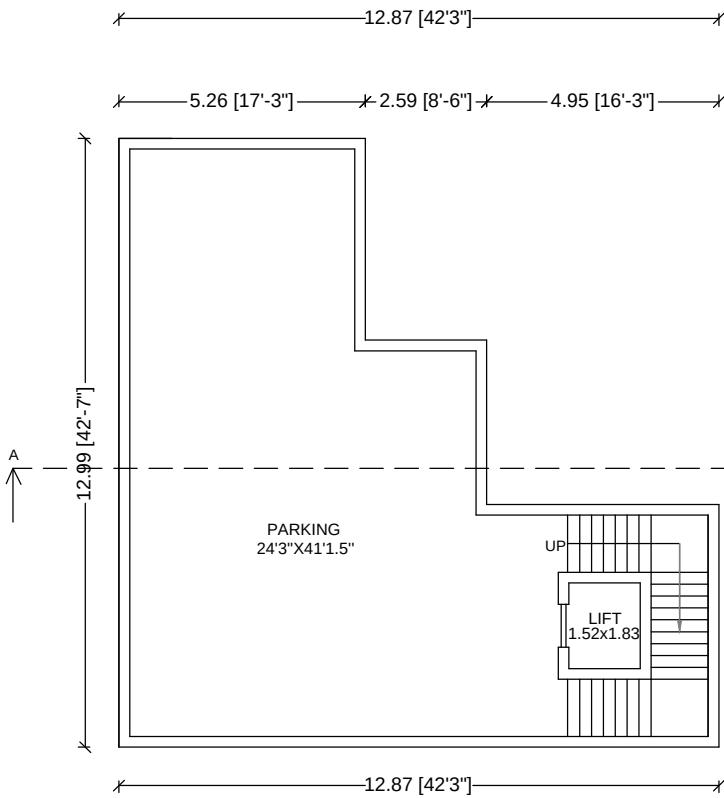
STILT FLOOR PLAN
