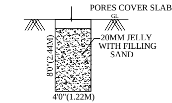
RAIN WATER HARVESTING UNIT
