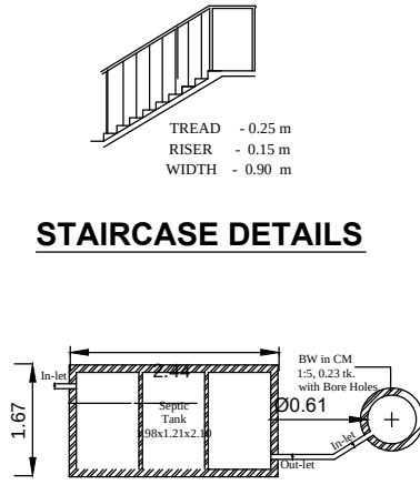
PLAN - SEPTIC TANK & SOAK PIT
