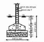
COLUMN FOUNDATION DETAIL
