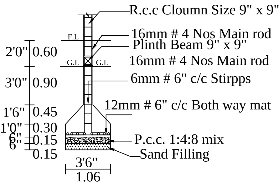
COLUMN DETIAL
