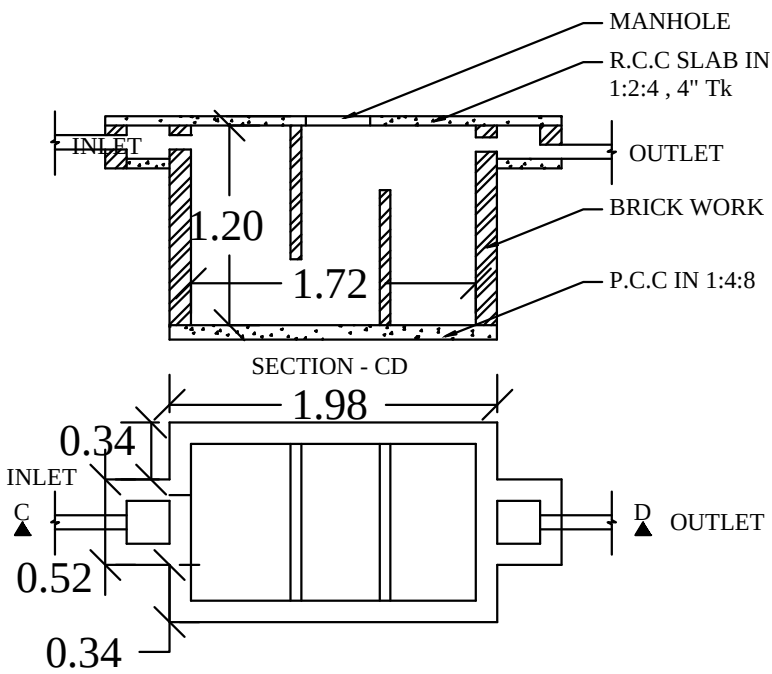
PLAN OF SEPTICK TANK
