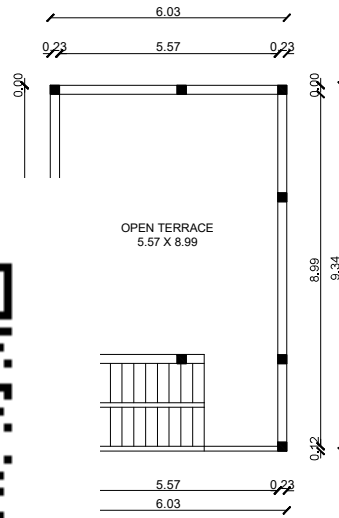
SED OPEN TERRACE FLOOR PLAN
