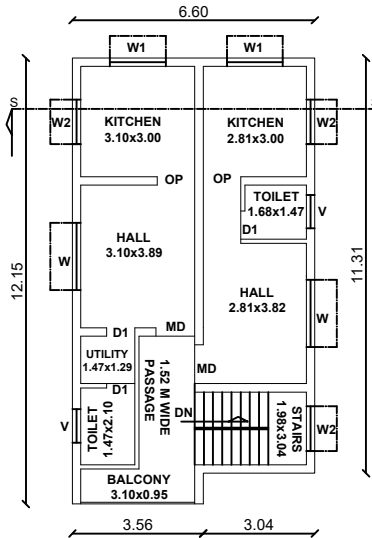
SECOND FLOOR PLAN (PRO)
