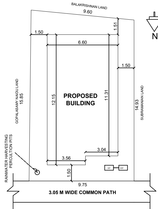
SITE PLAN
