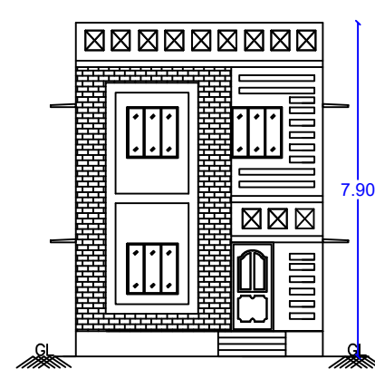
FRONT ELEVATION
