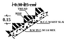
STAIRCASE SECTION
