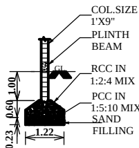
COLUMN DETAILS
