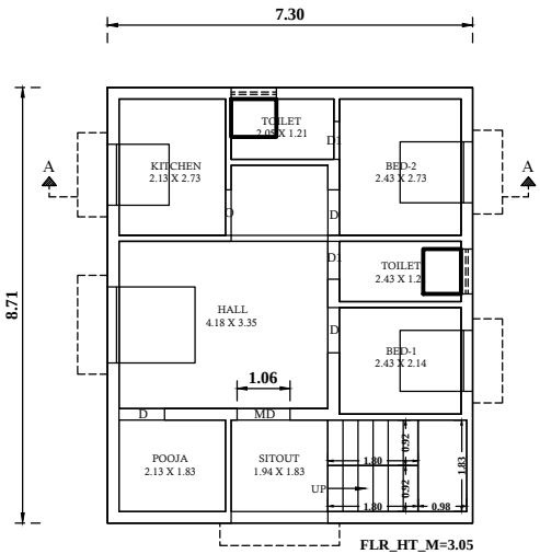
PRO FIRST FLOOR
