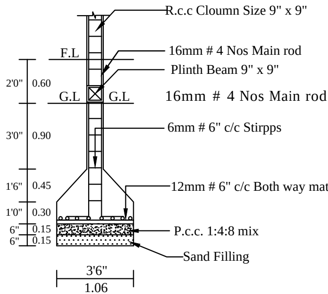
COLUMN DETIAL
