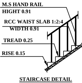
STAIRCASE DETAIL
