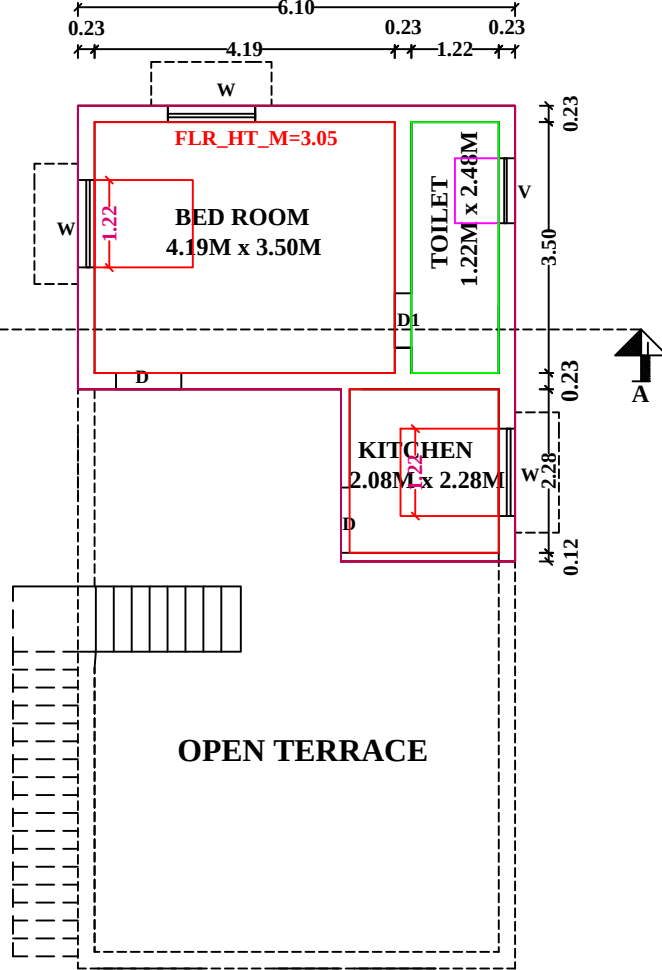
FLOOR-0
