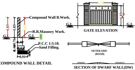
SECTION OF DWARF WALL(DW)
