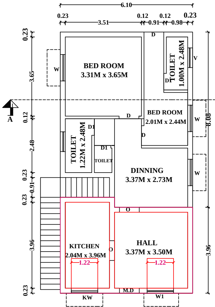
FLOOR-GROUND
