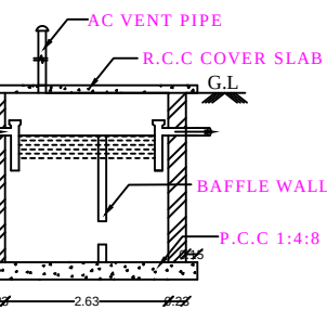
SAEPTIC TANK DETAILS
