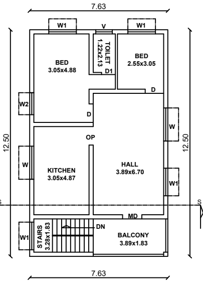
SECOND FLOOR PLAN (PRO)
