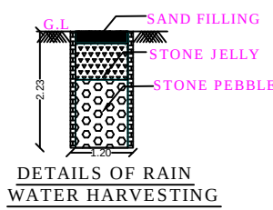
DETAILS OF RAIN WATER HARVESTING
