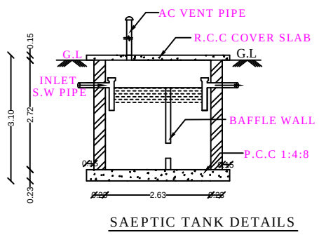
SAEPTIC TANK DETAILS
