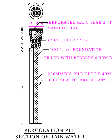
PERCOLATION PIT SECTION OF RAIN WATER
