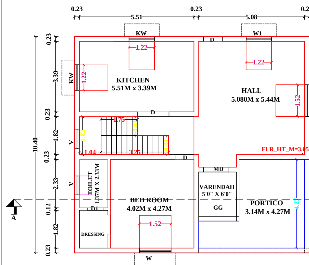
FLOOR-0 PRO.GROUND FLOOR PLAN
