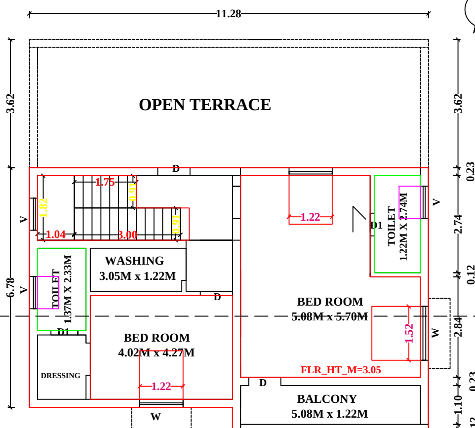
FLOOR-1 PRO.FIRST FLOOR PLAN
