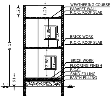
SECTION ON XX
