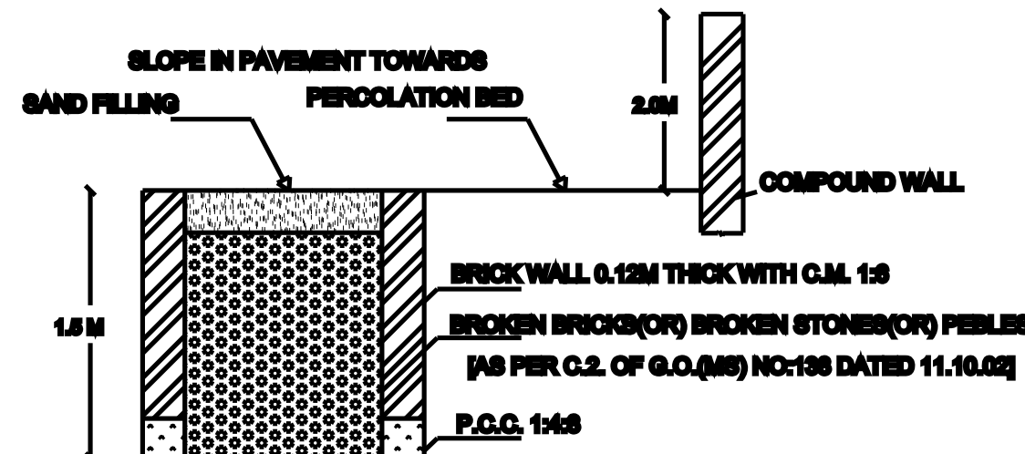
SECTION OF RAIN WATER PERCOLATION BED
