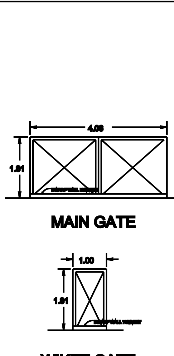
MAIN GATE
