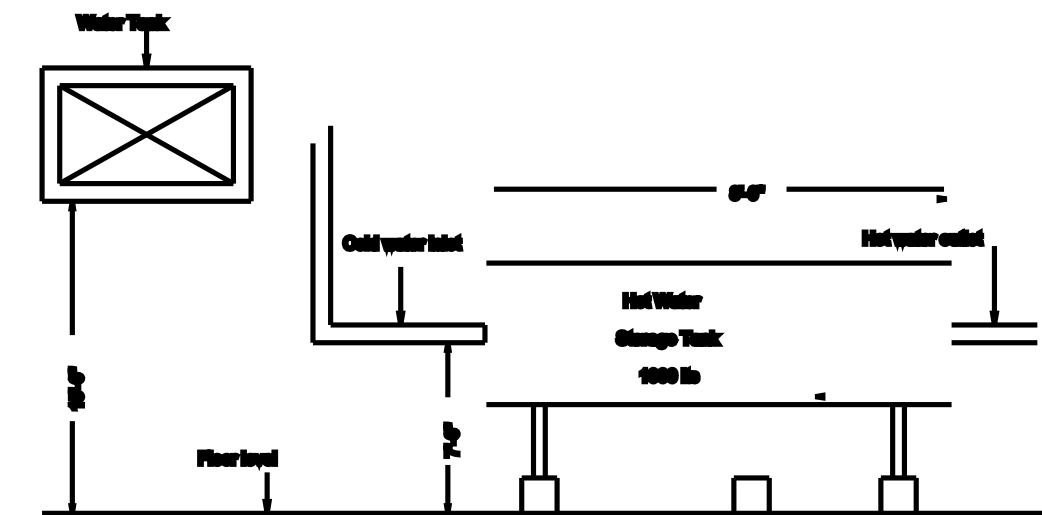
SOLAR WATER HEATER DETAILS
