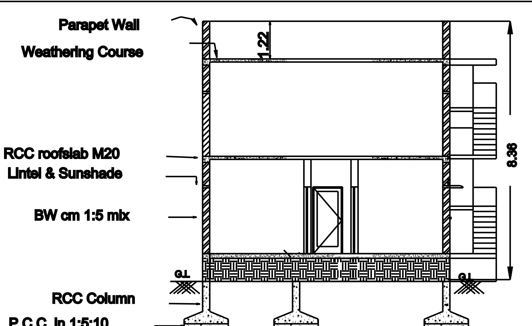
SECTION- BB
