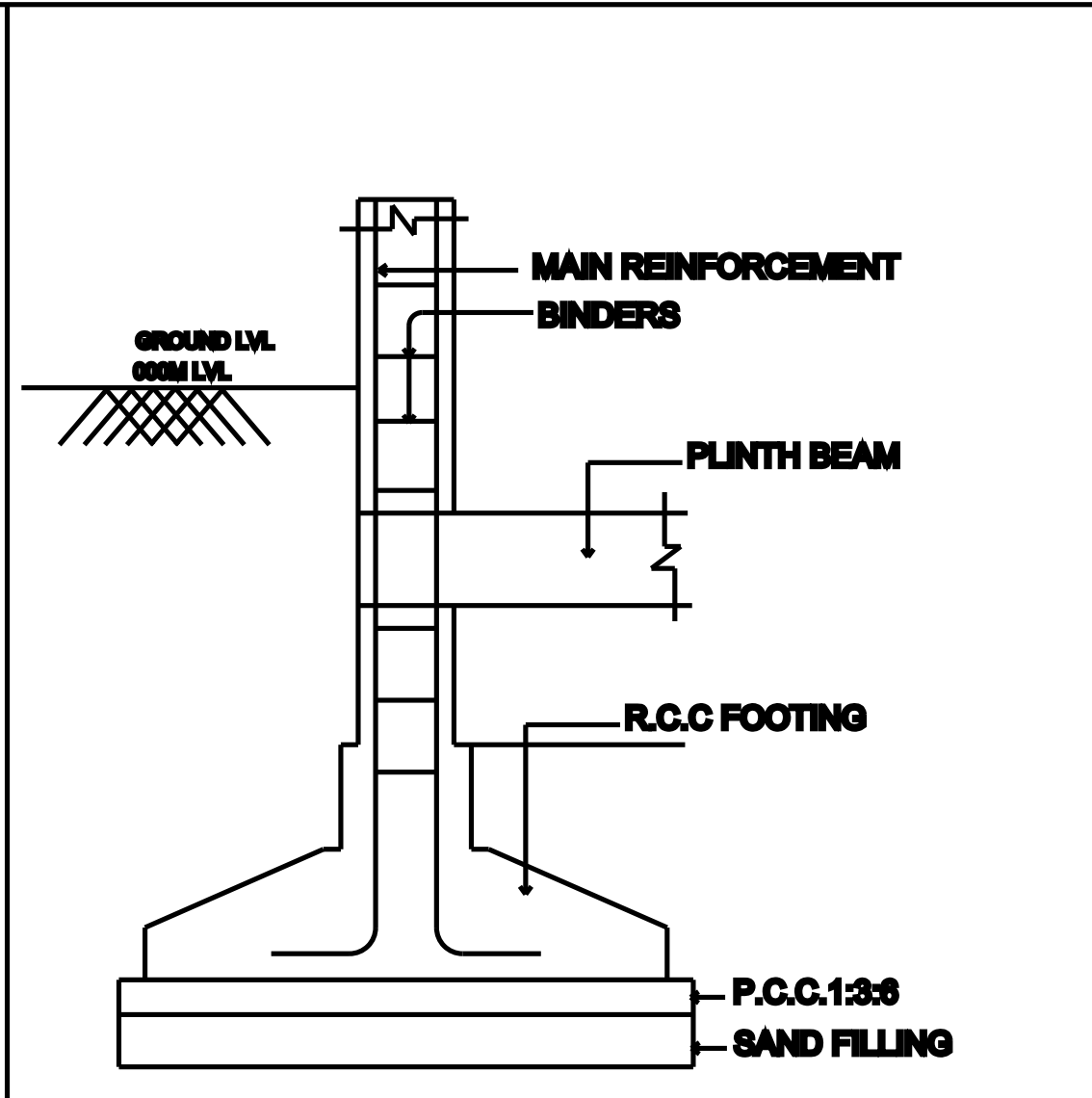
TYPICAL SECTION OF R.C.C COLUMN FOUNDATION
