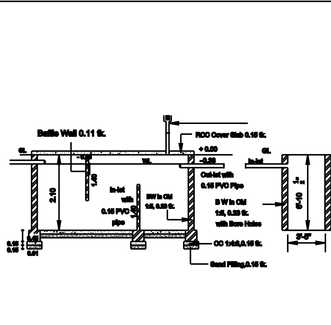
SECTION - SEPTIC TANK & SOAK PIT
