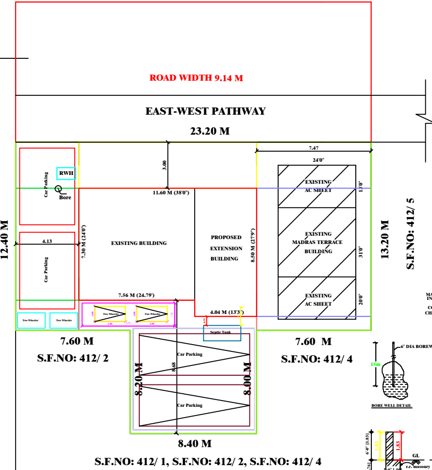
SITE PLAN
