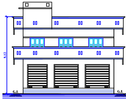
FRONT ELEVATION
