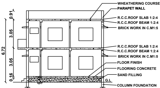
SECTION ON GG
