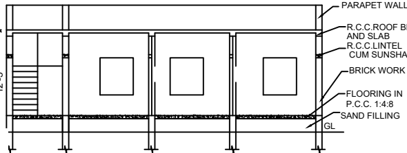
SECTION AB
