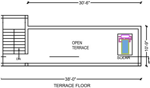
TERRACE FLOOR
