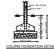
COLUMN FOUNDATION DETAIL
