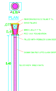
SECTION OF RAIN WATER RWH_CAPACITY_1=500
