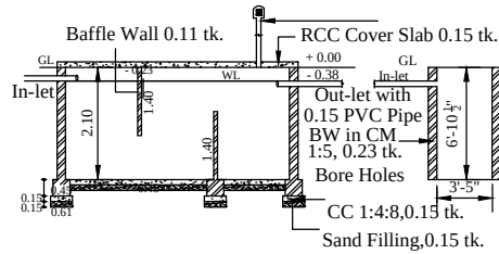
SEPTIC TANK & SOAK PIT
