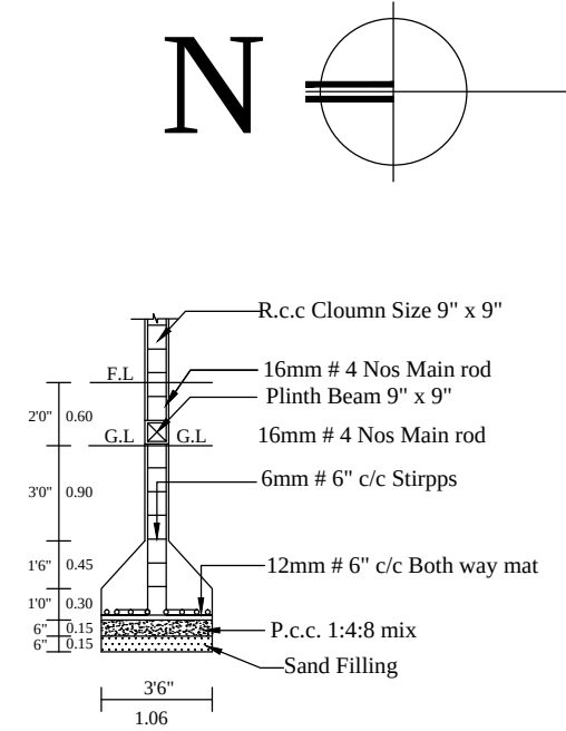
COLUMN DETIAL
